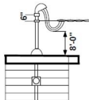
Flat Roof NEC 230.24 A(3)
